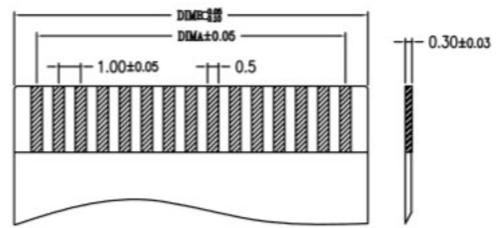
APPLICABLE FPC/FFC DIM. (THICKNESS 0.30±0.02)
